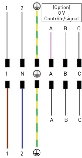
RETTBOX® ONE 32 A/230 V
