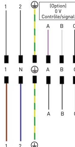
RETTBOX® ONE AIR 32 A/230 V
