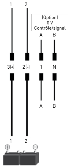
RETTBOX® ONE 20 A 12/24 V
